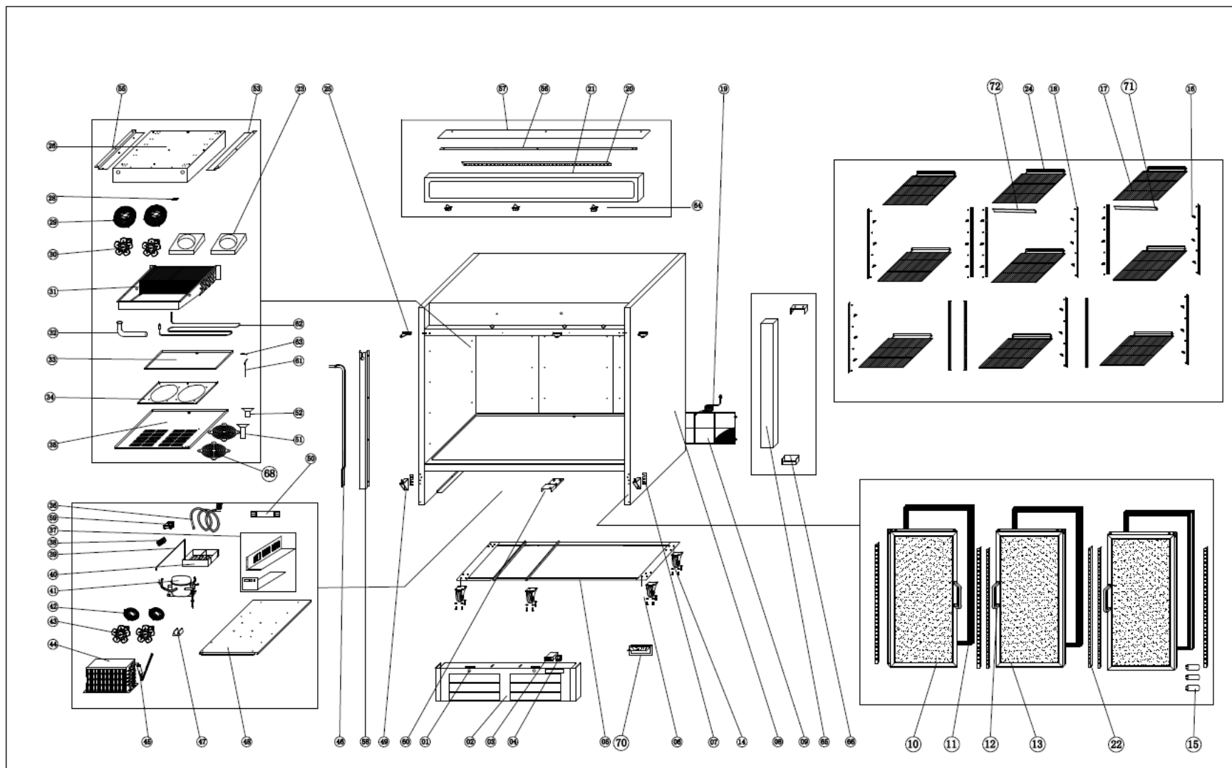
EXPLODE OF KCHGM72F (R404a Version)
